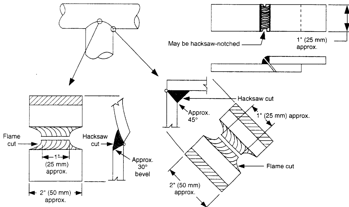
Figure 11—Location of Nick-Break Test Specimens: Fillet-Weld Procedure and Welder Qualification Test Welds, Including Size-to-Size, Branch-Connection Welder Qualification Test
