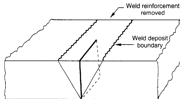
Figure A-3—Location of Notch for Weld-Metal Specimen
