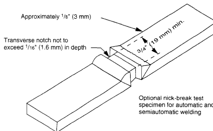
Figure 5—Nick-Break Test Specimen
