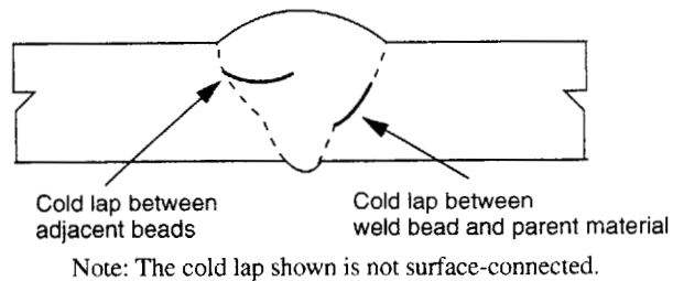
Figure 17—Incomplete Fusion Due to Cold Lap (IFD)
