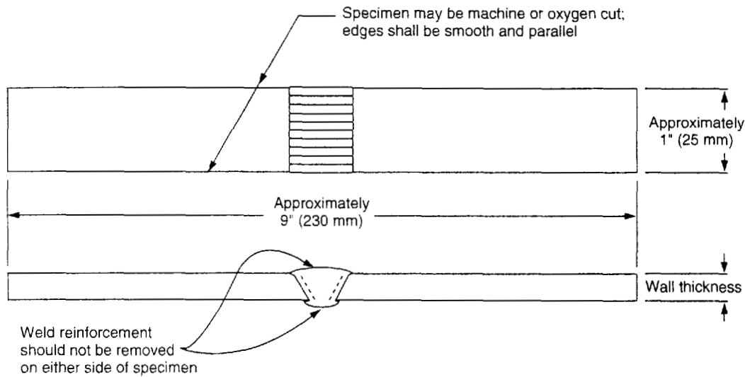
Figure 4—Tensile-Strength Test Specimen
