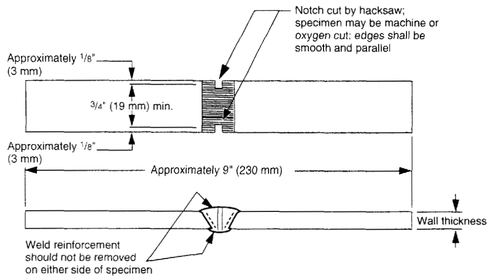
Figure 4—Tensile-Strength Test Specimen
