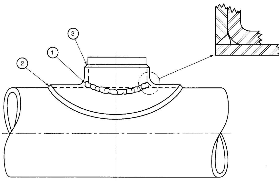
Figure B-7—Reinforcing Saddle
